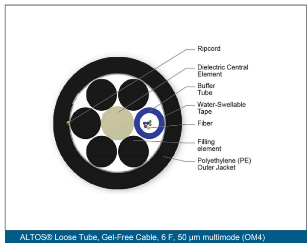
ALTOS® Loose Tube, Gel-Free Cable, 6 F, 50 µm multimode (OM4)
