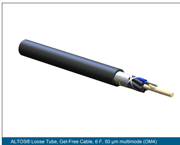
ALTOS® Loose Tube, Gel-Free Cable, 6 F, 50 µm multimode (OM4)
